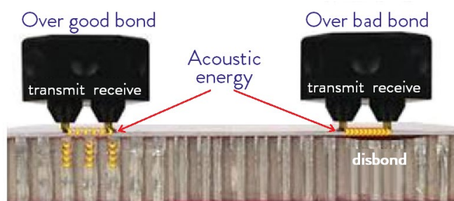
Figure 39: Pitch-catch. Image: MTD Group (adapted)
