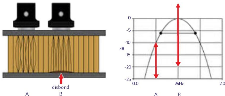
Figure 37: Membrane resonance. Image: MTD Group (adapted)
