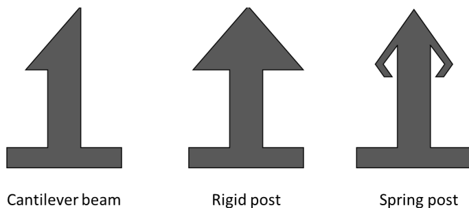
Figure 8: Three examples of locking features for mechanical attachment (Adapted from Messler, 1997 5 )
